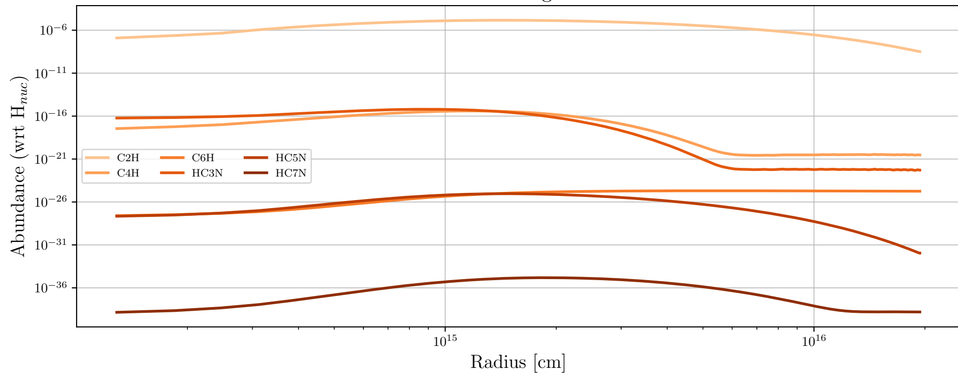
Particle 33138 - Daughter Molecules
