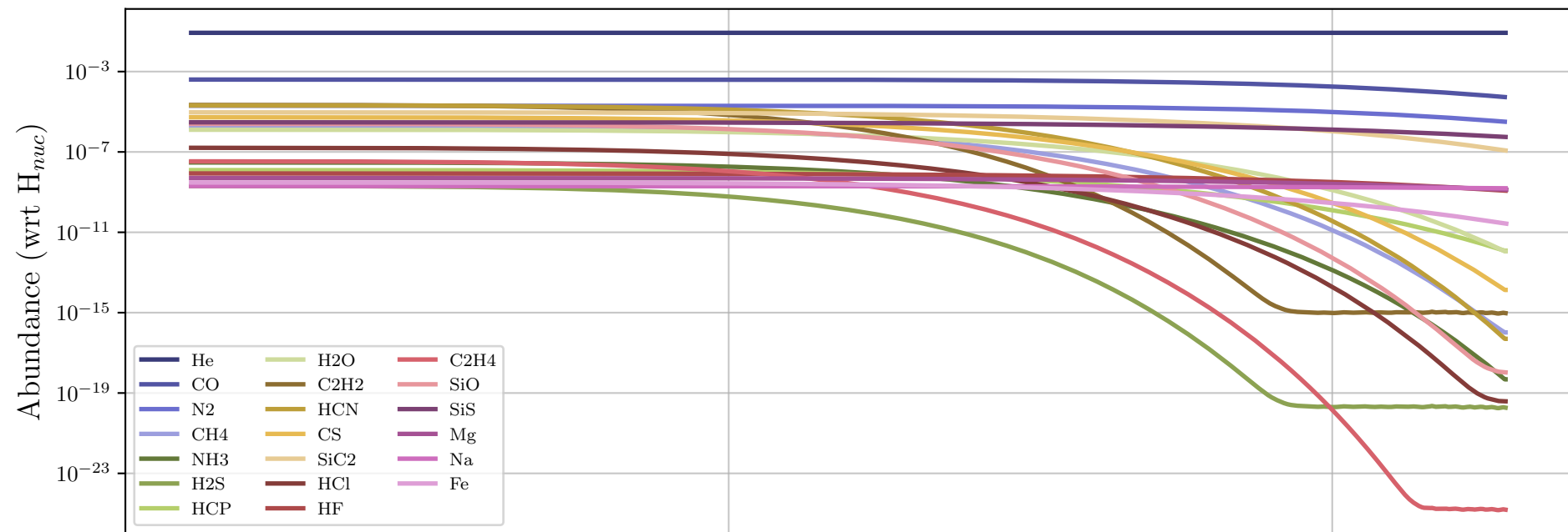
Particle 33138- Parent Molecules
